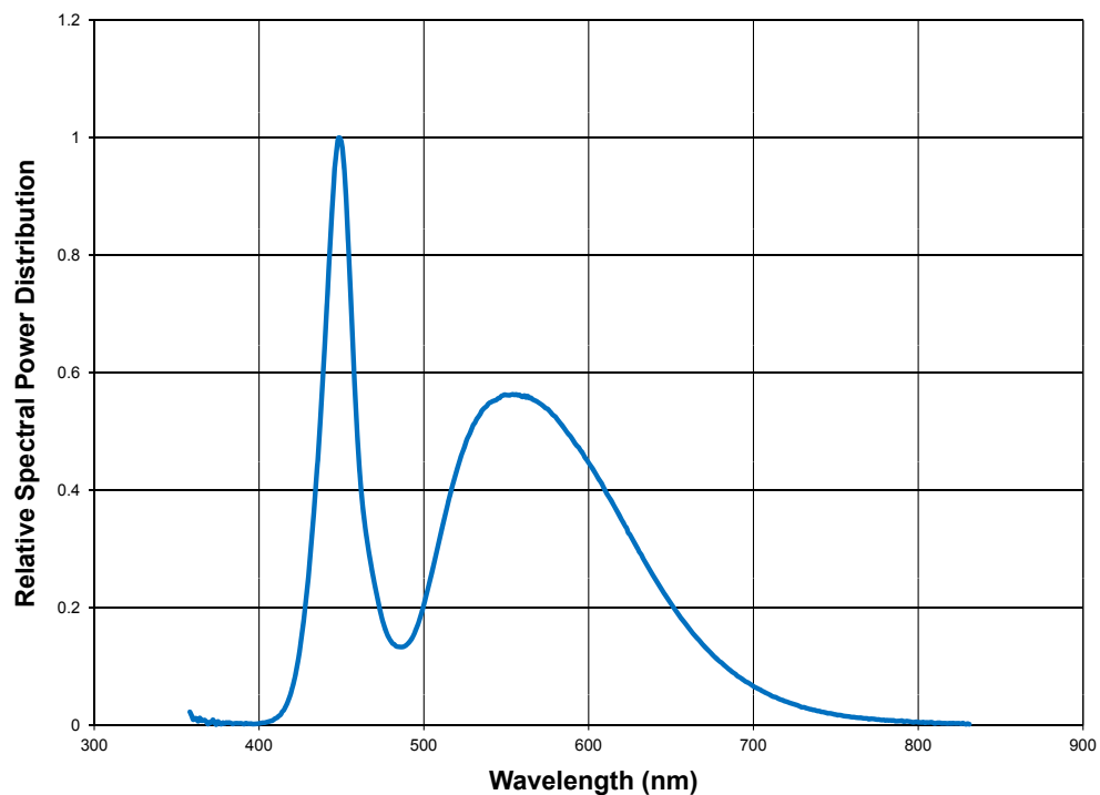
Figure 5. White color spectrum of typical CCT part, integrated measurement.
